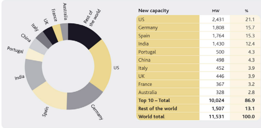
TOP 10 NEW INSTALLED CAPACITY (JAN.-DEC. 2005)
