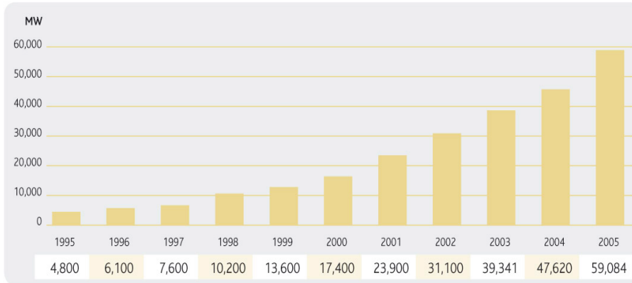
GLOBAL CUMULATIVE INSTALLED CAPACITY 1995-2005
